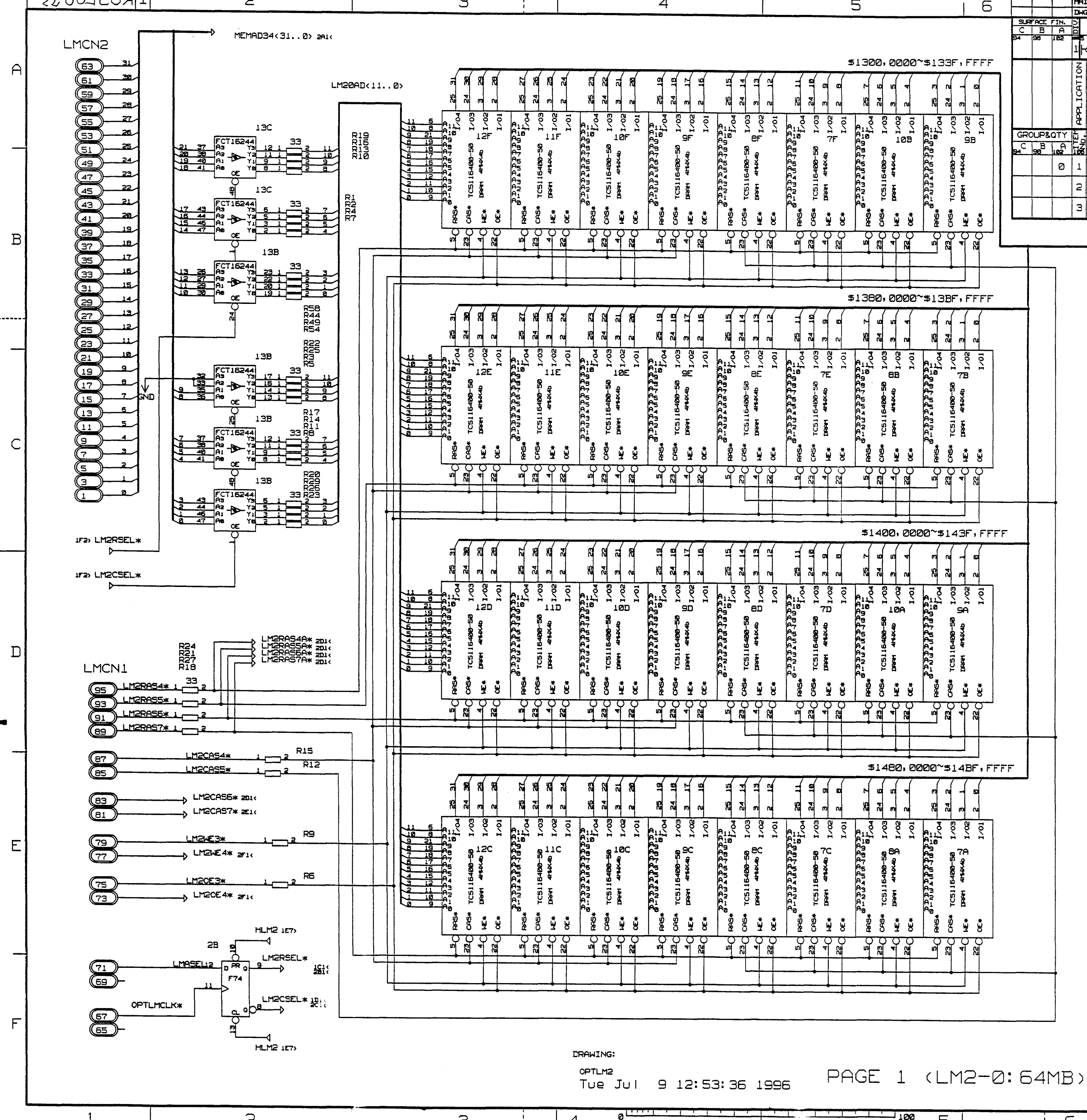
MRDM CIRCUIT DIAGRAM(1/3)
