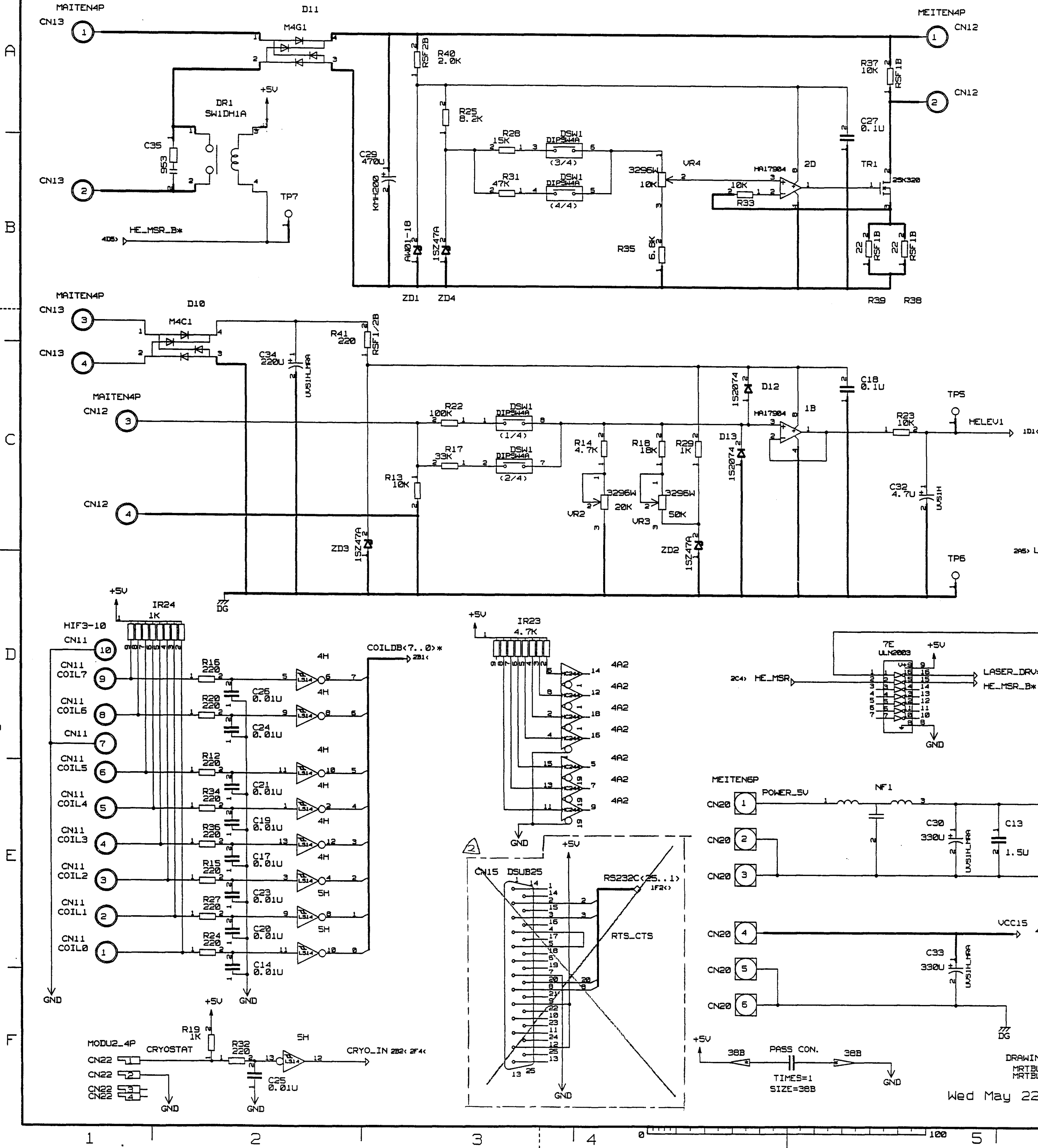
I/F & POWER_SUPPLY TCONT3 CIRCUIT DIAGRAM (4/7)
