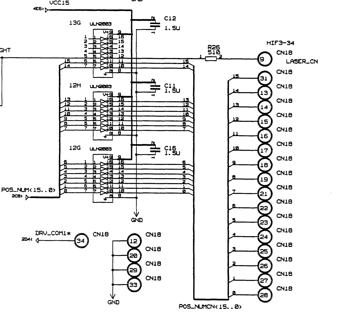
I/F & POWER_SUPPLY TCONT3 CIRCUIT DIAGRAM (4/7)
